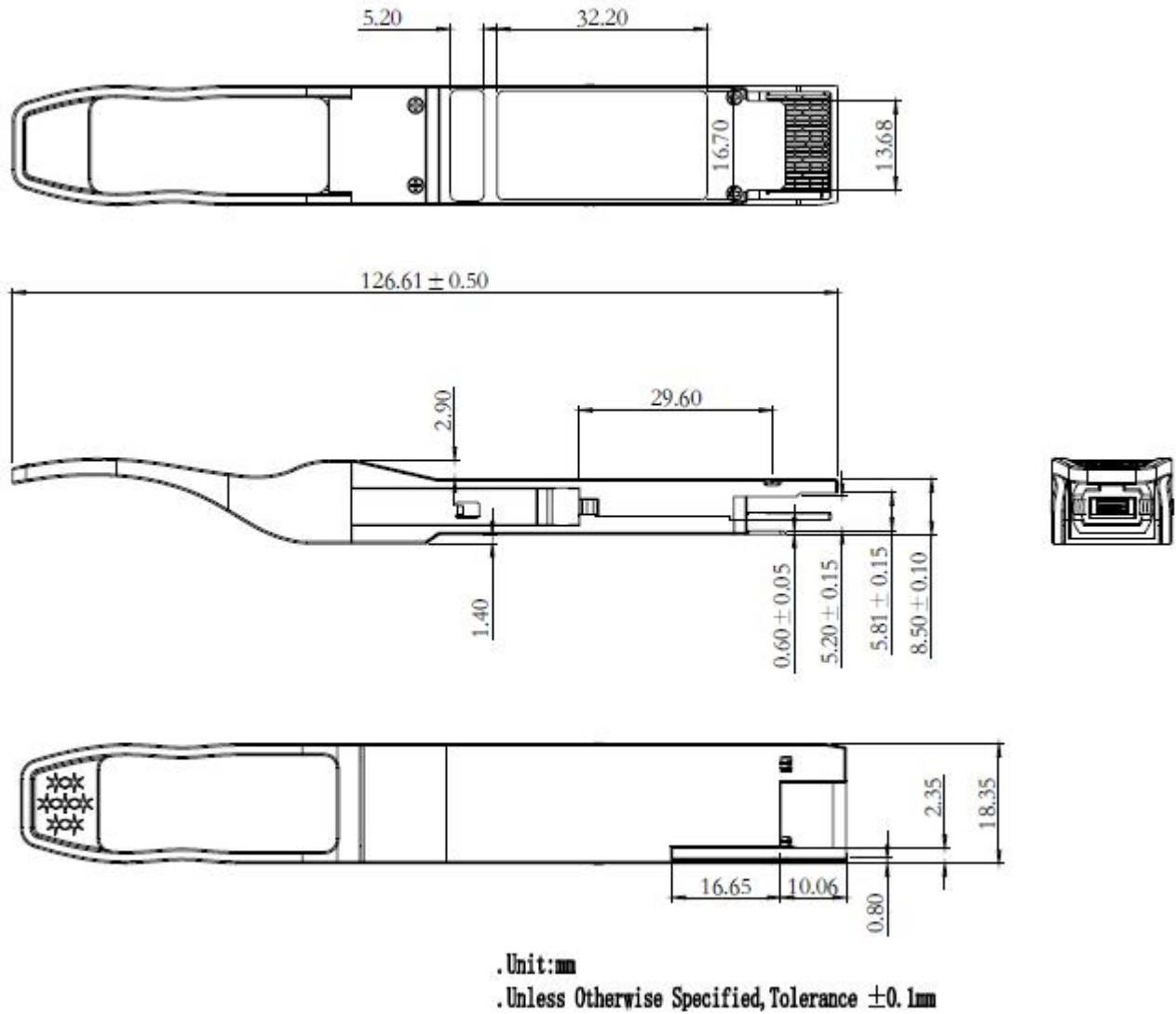
Figure 9. Mechanical Specifications
