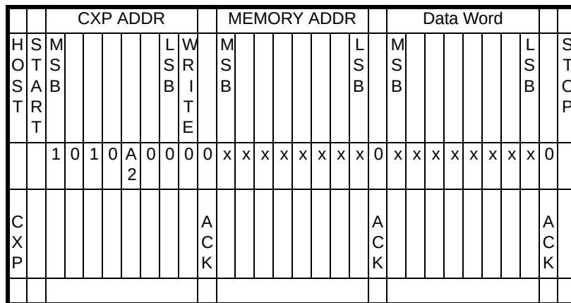
Figure 35 Write Byte Operation
