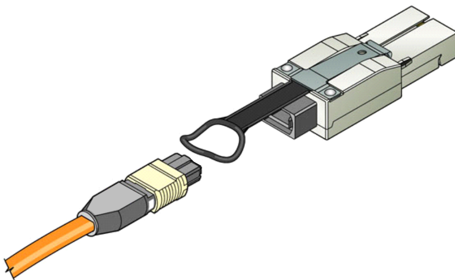
Figure 22 Optical Transceiver with separable optical cable
