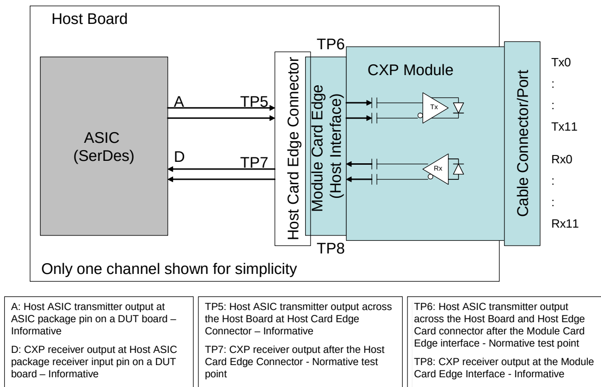
Figure 4 Application Reference Model and Compliance Points
