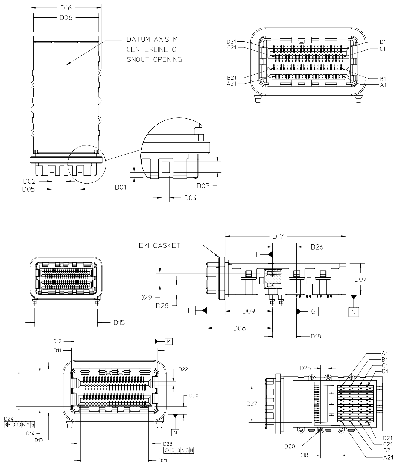
Figure 10 Fixed (Receptacle) Connector
