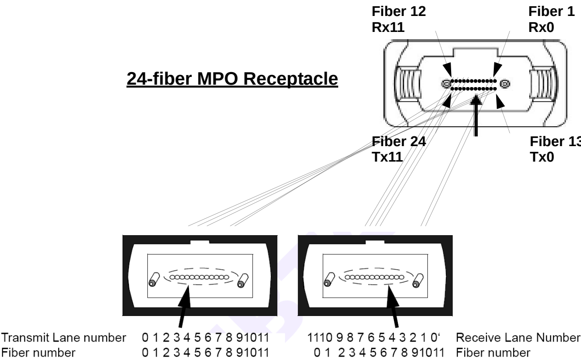
Figure 28 Connector interface between 24-fiber and Two 12-fiber connectors
