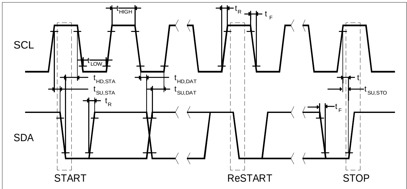
Figure 29 CXP 2-wire Serial Interface Timing Diagram
