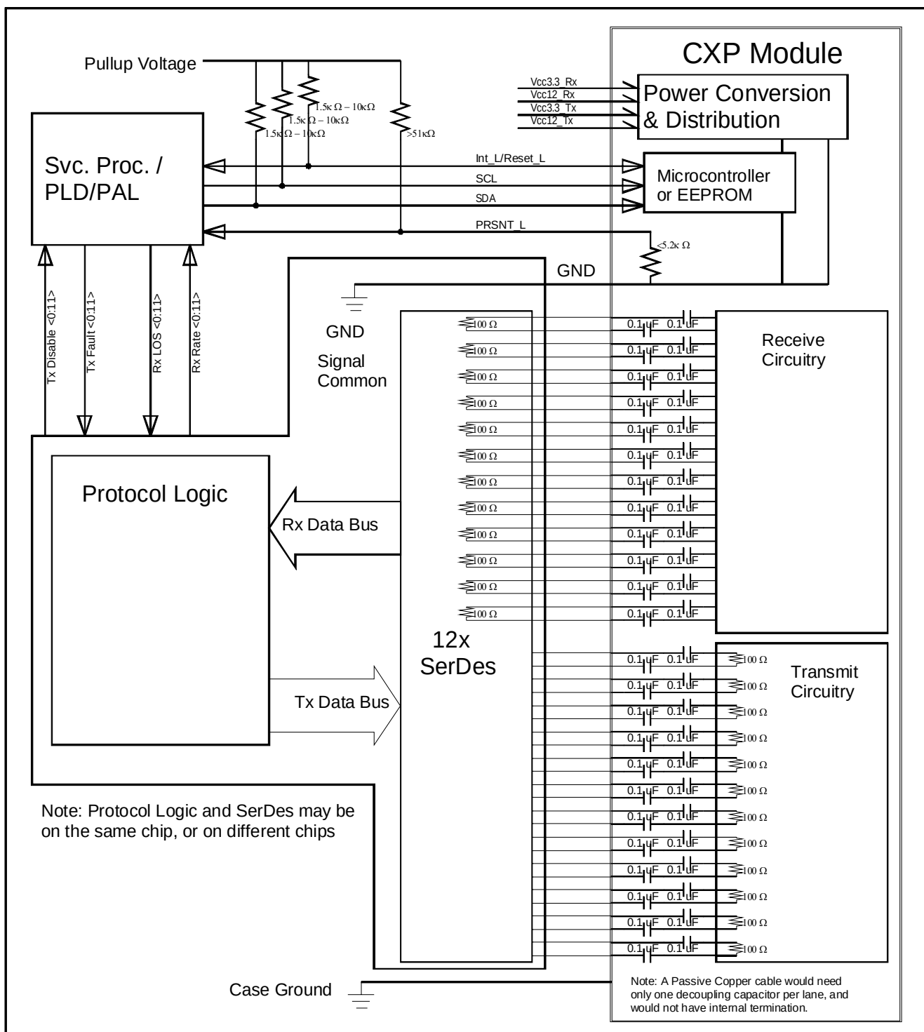
Figure 2 Example Host Board Schematic
