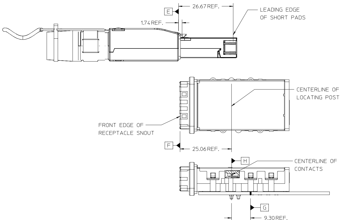
Figure 6 Cable Connector and Receptacle Housing Datums
