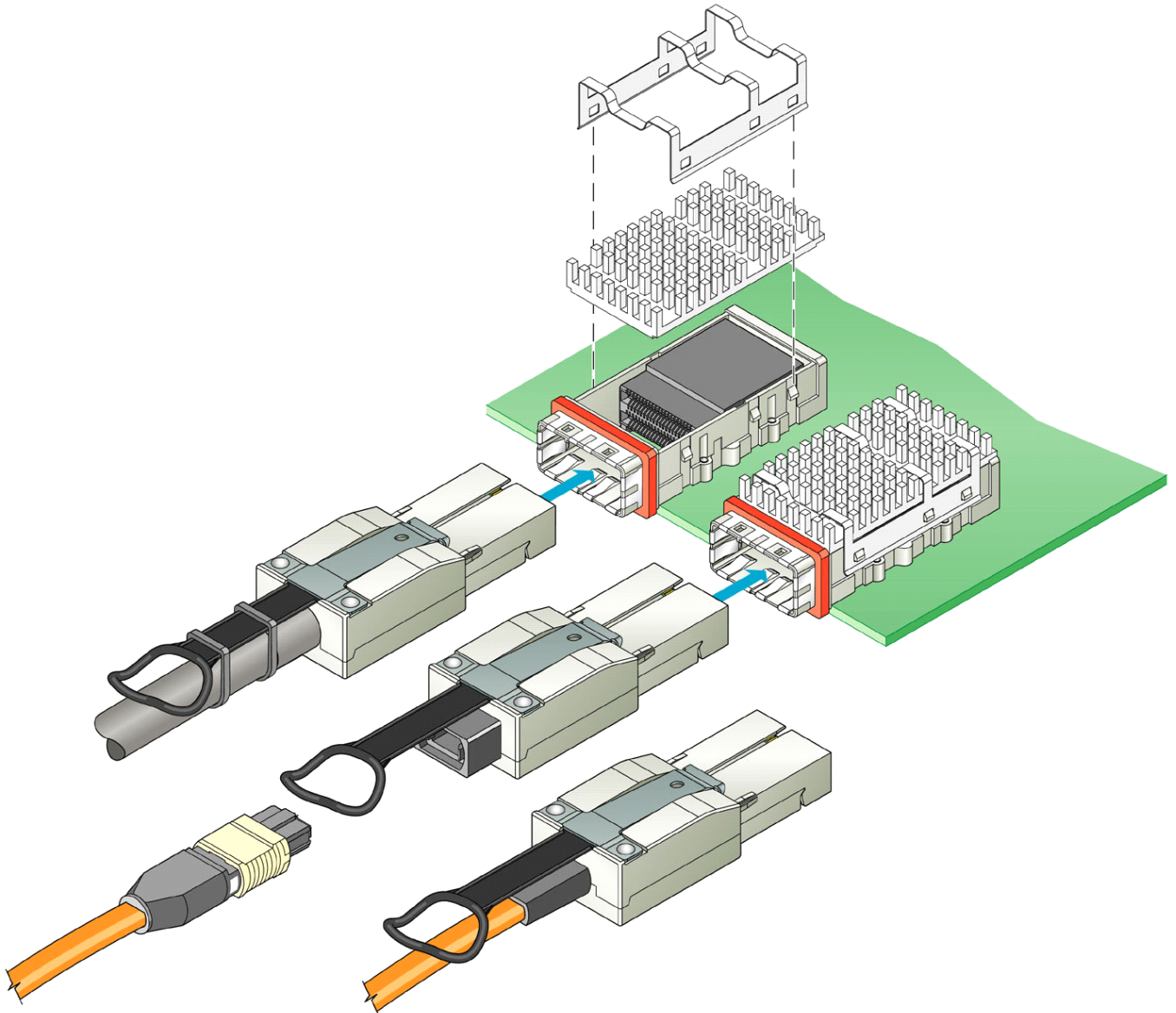
Figure 1 CXP Conceptual Model
