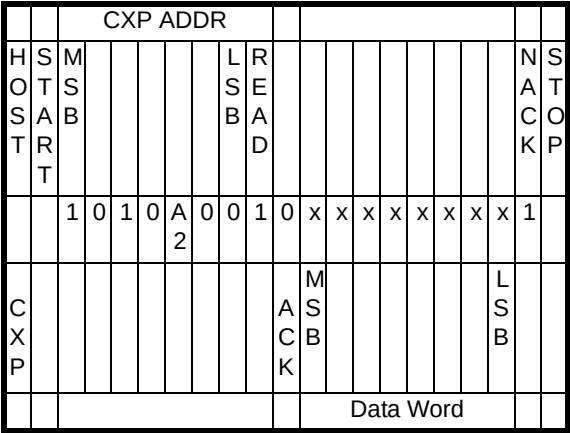
Figure 31 Read Operation on Current Address
