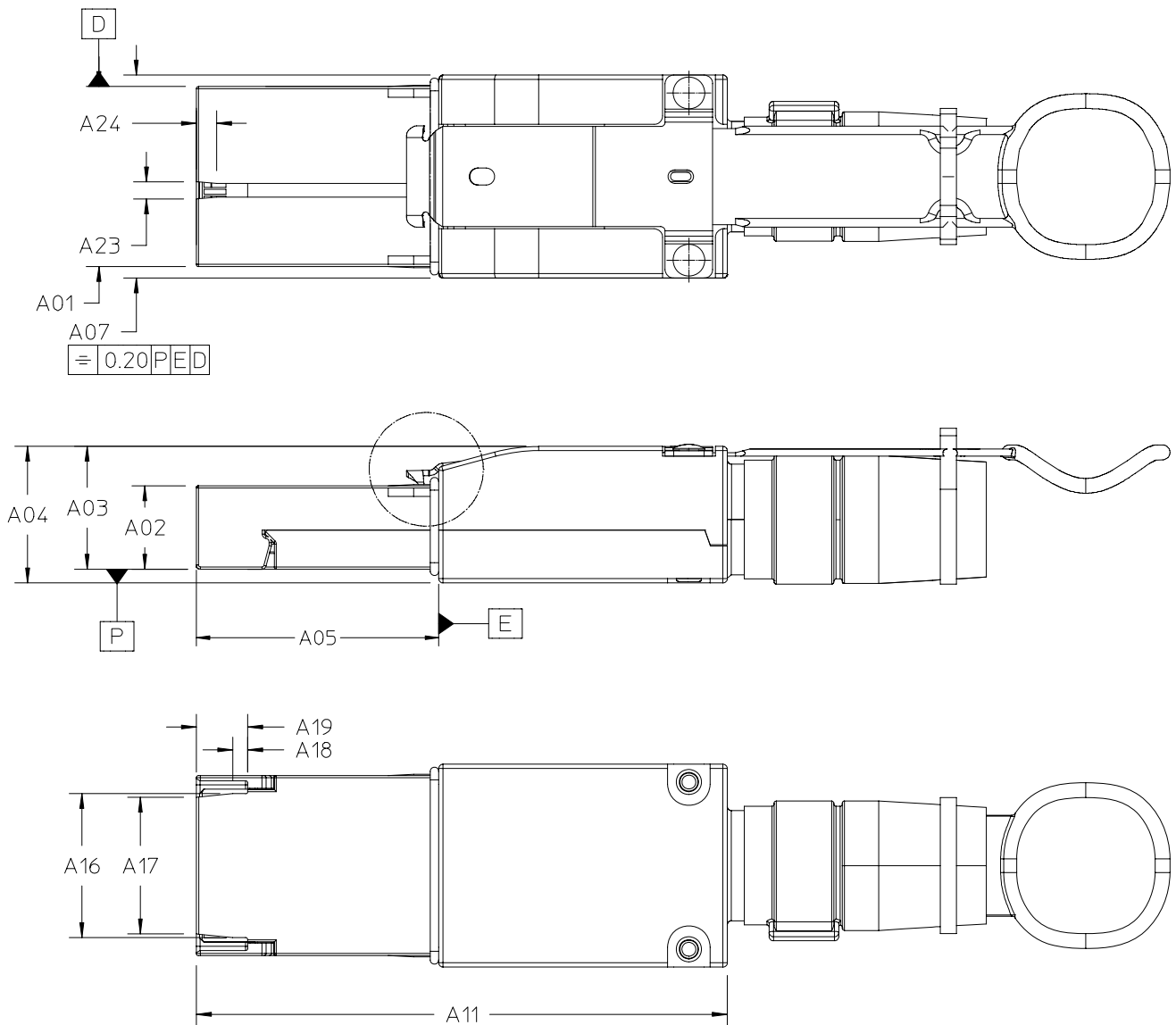
Figure 7 Shielded Free (Plug) Integrated Cable Connector
