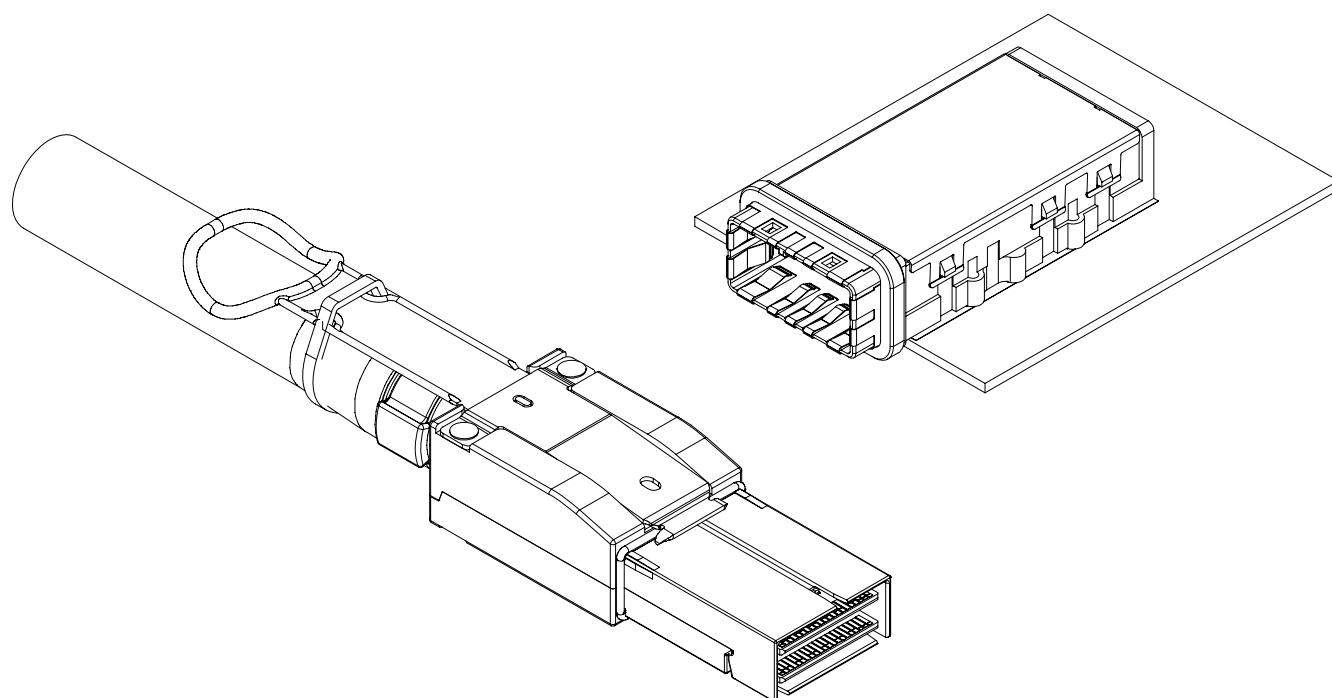
Figure 5 General view, CXP Cable Connector & Housing Assembly, w/o heat sink
