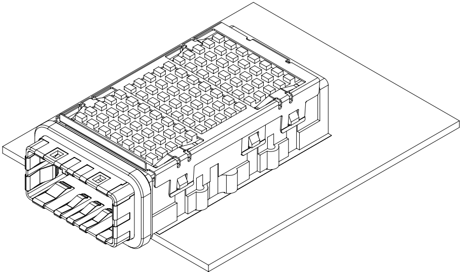
Figure 16 Receptacle Housing with Integrated Riding Heat Sink
