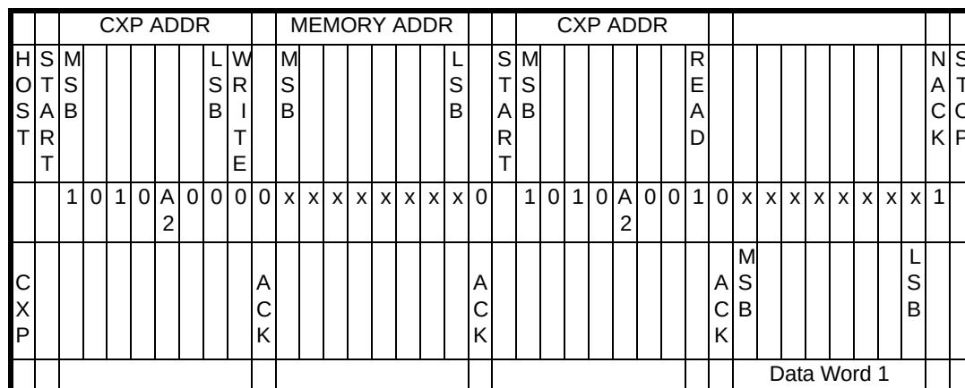
Figure 32 Random Read
