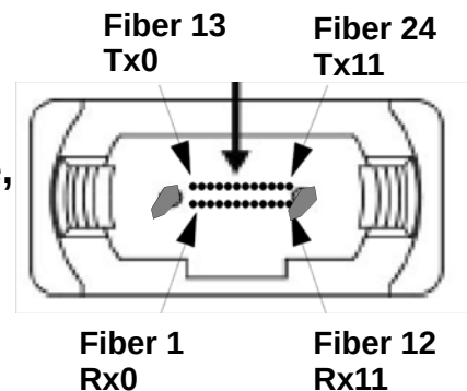
Figure 27 Connector orientation for 24-fiber MPO/MTP connector
