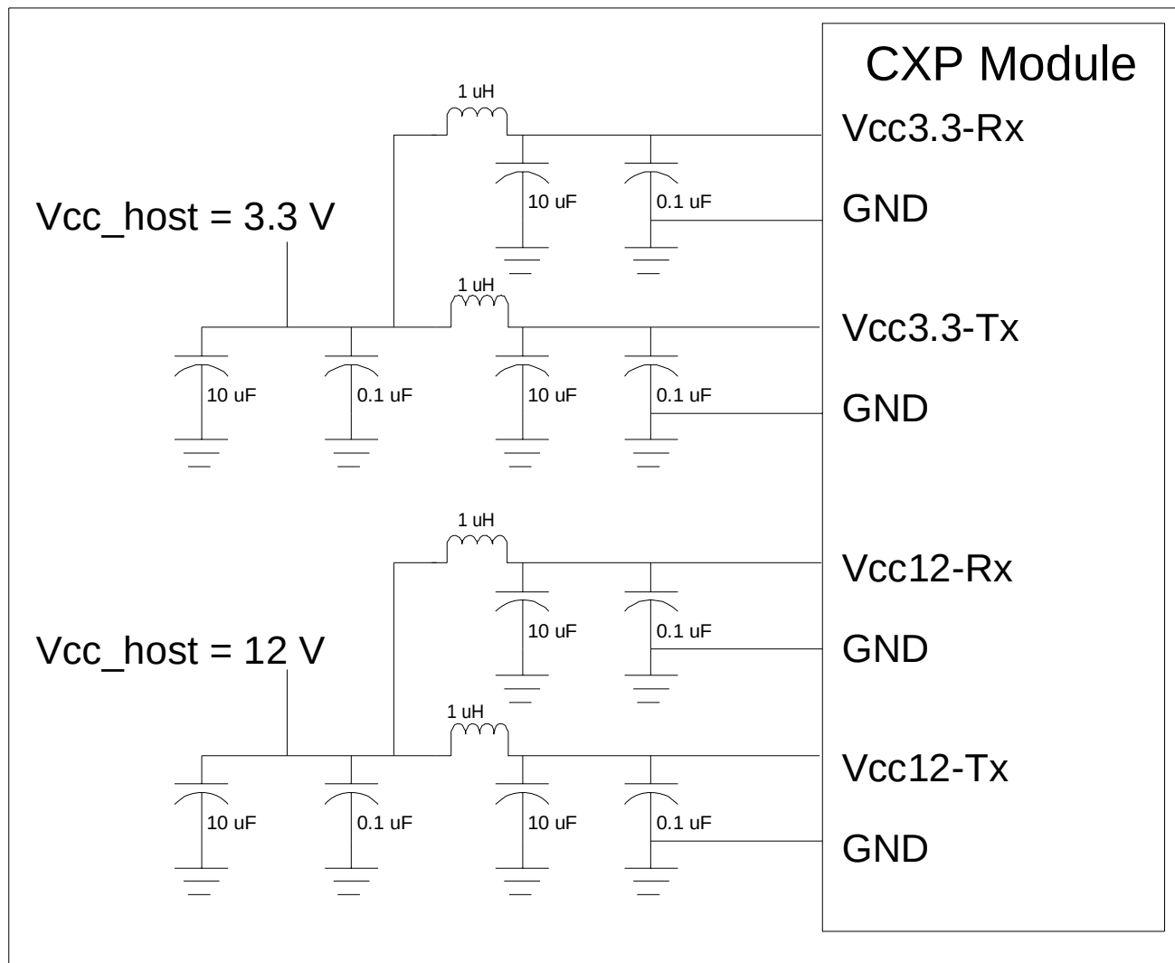
Figure 3 Recommended Host Board Power Supply Filtering
