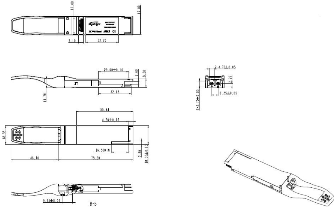
Figure9. Mechanical Specifications
