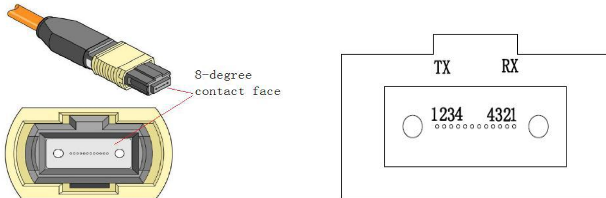
Female MPO(APC 8-degree) connector for this module
