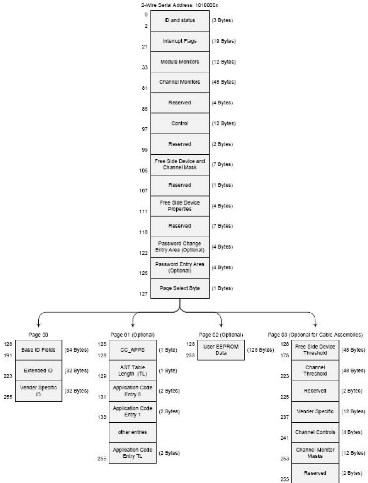
Figure5.QSFP Memory Map
