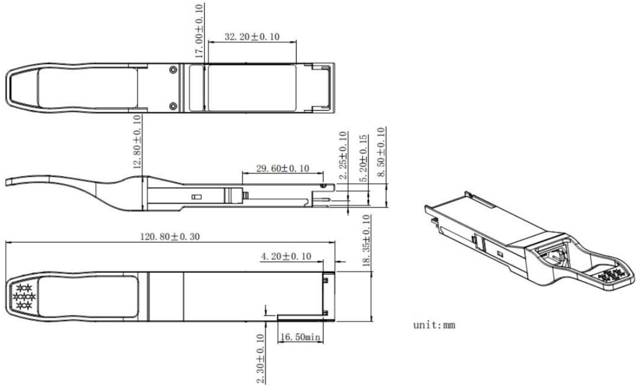
Figure10. Mechanical Specifications
