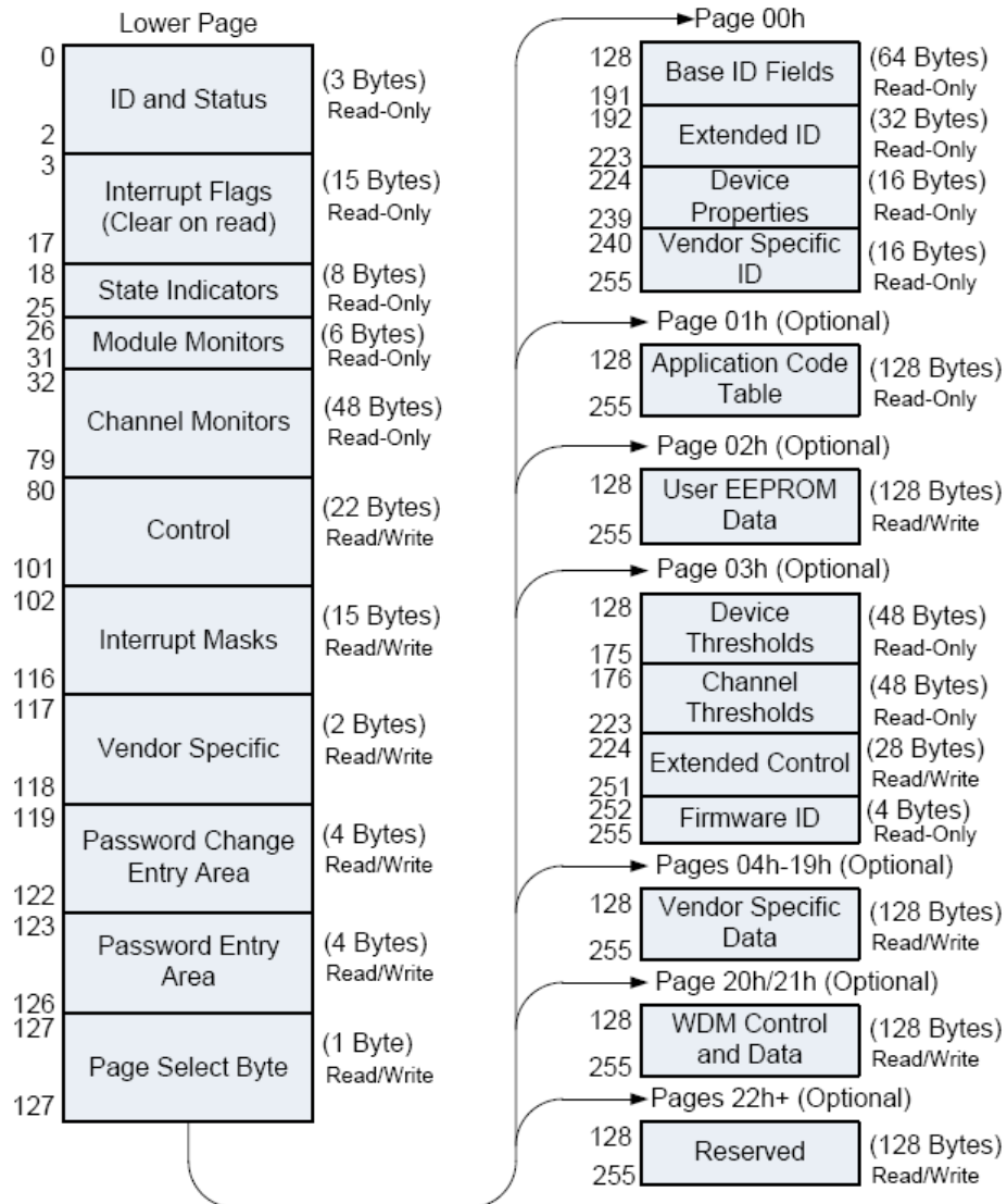
Figure 5. QSFP DD Memory Map
