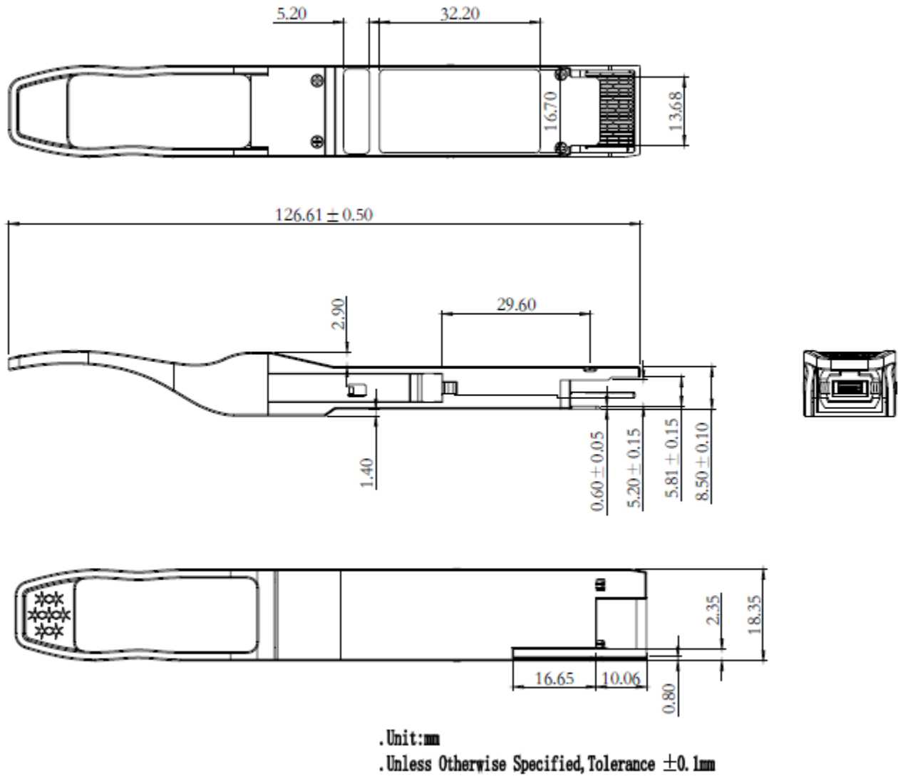
Figure 9. Mechanical Specifications
