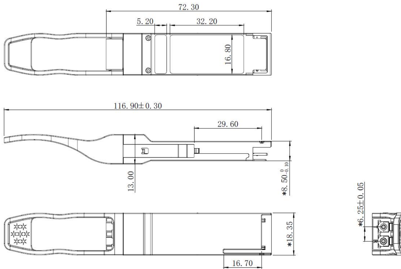
Figure 12. Mechanical Specifications
