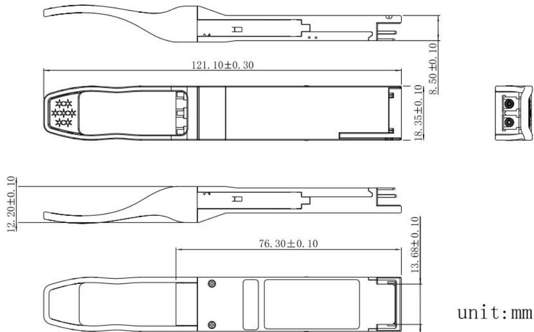
Figure 8. Mechanical Specifications
