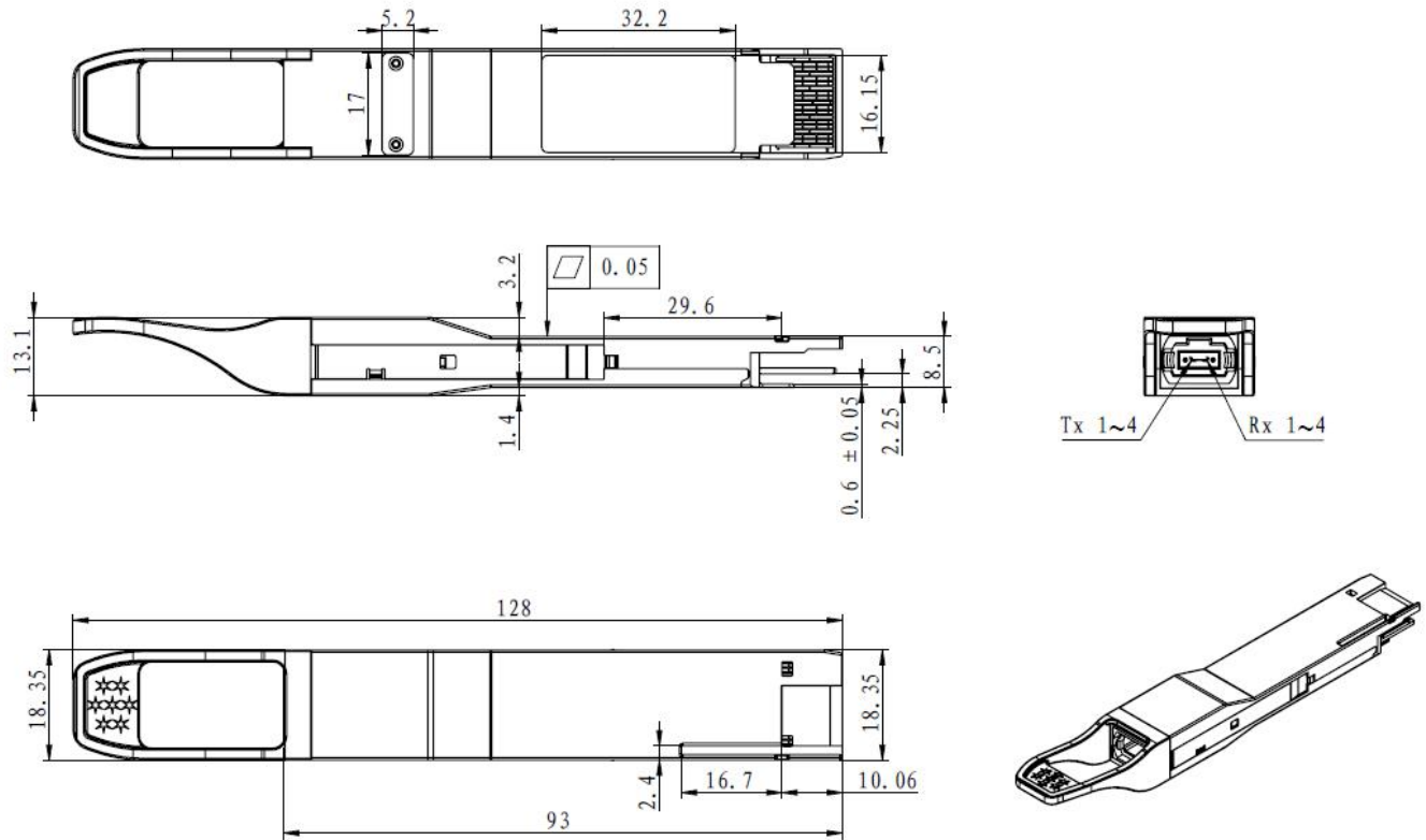
Figure5. Mechanical Specifications
