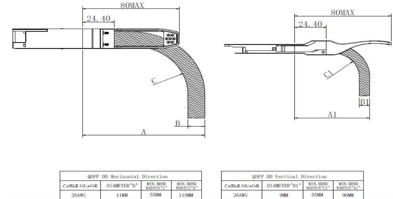
Figure 2. Mechanical Specifications
