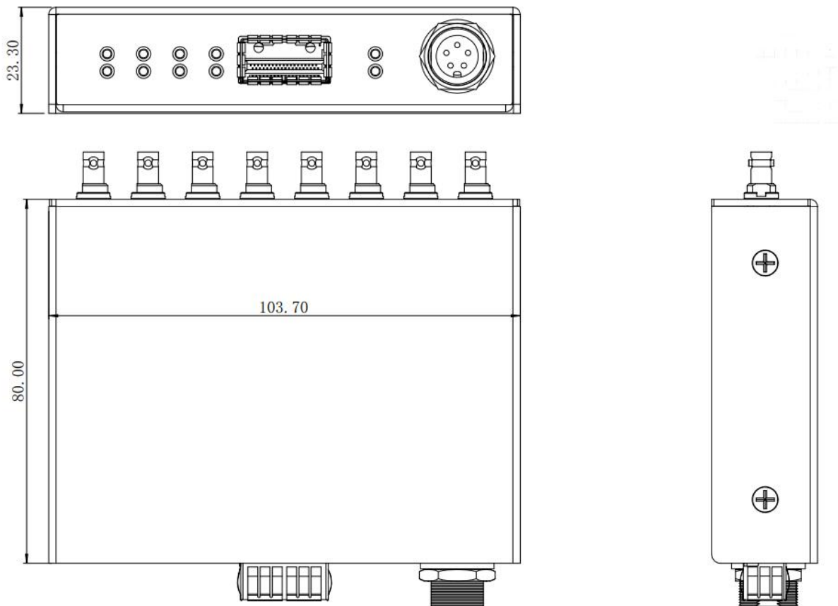
Figure 2. Mechanical Specifications (Power adapter not included)
