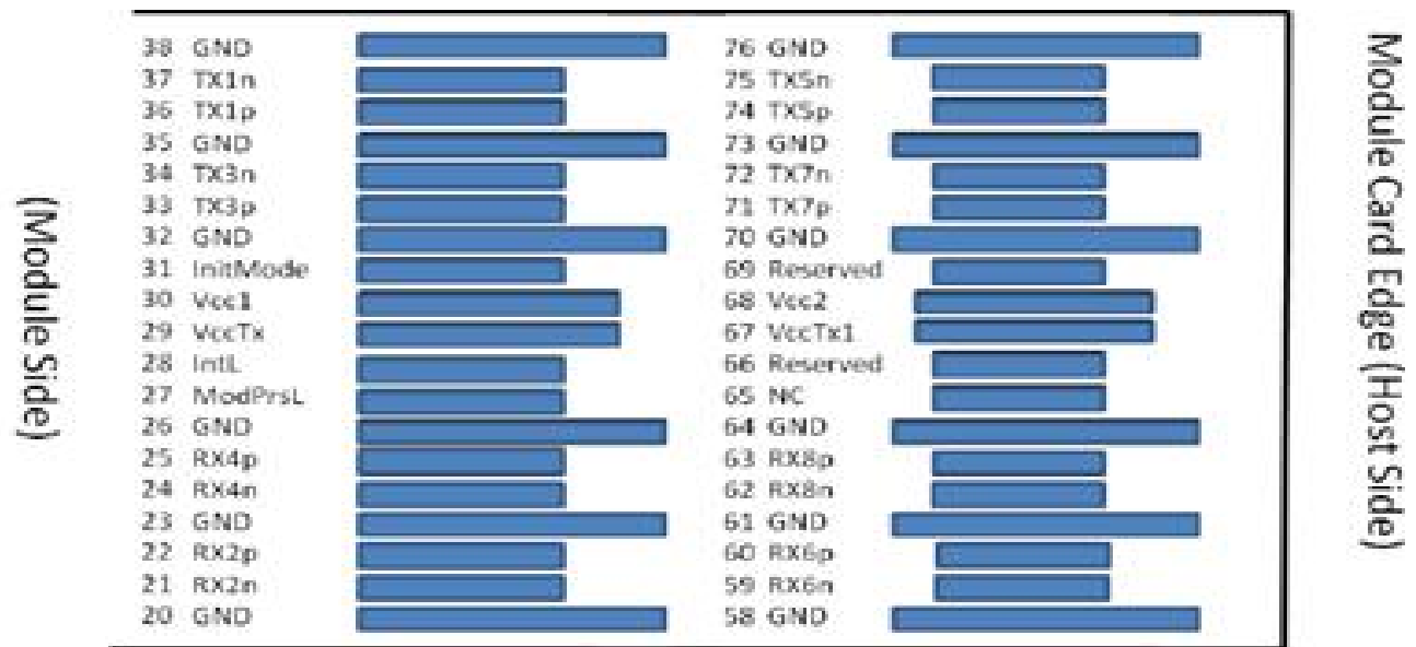
Top side viewed from top
