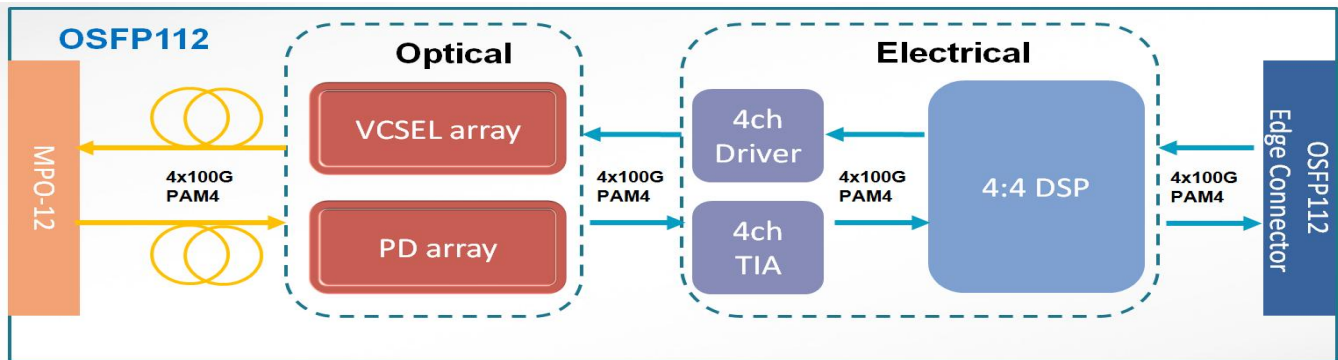
Figure 1. Module Block Diagram
