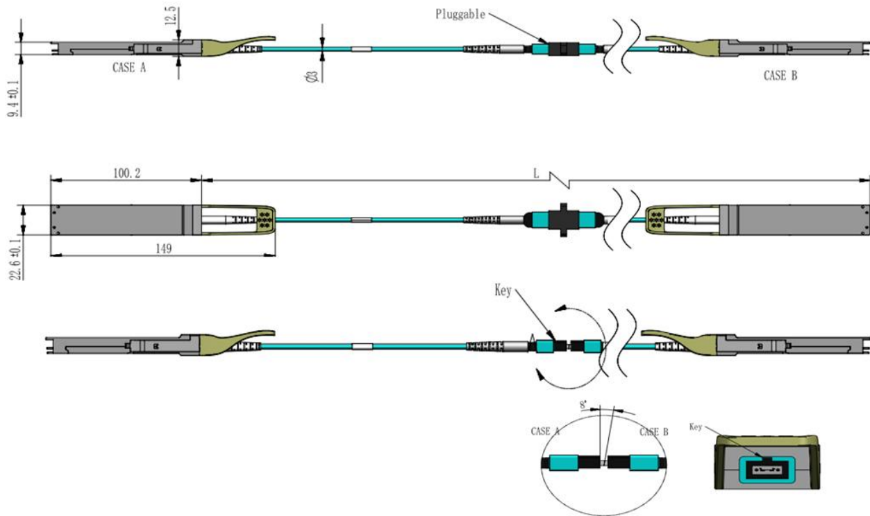
Figure 7. Mechanical Specifications
