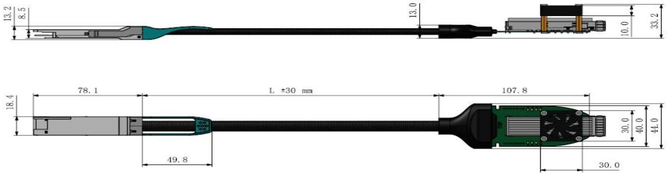
Figure 5. Mechanical Specifications
