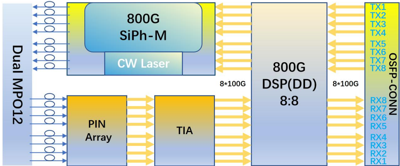
Figure1. DR8 Module Block Diagram
