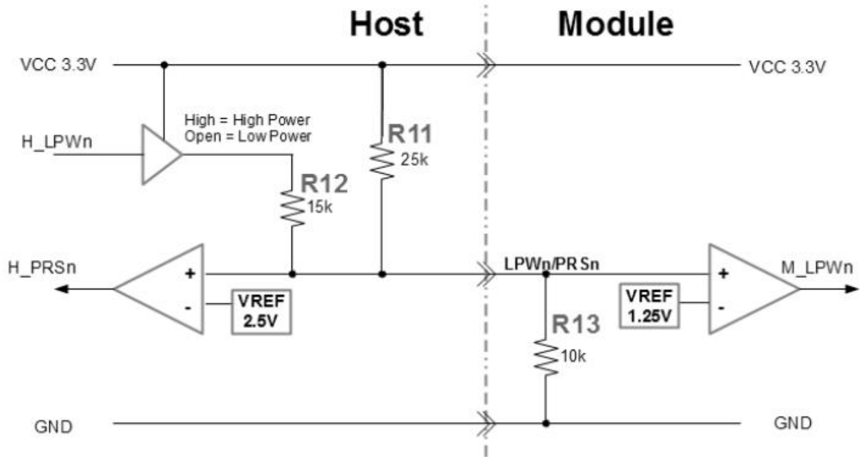
Figure 6. LPWn/PRSn circuit
