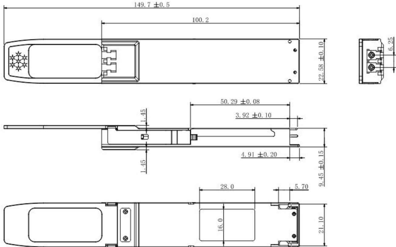
Figure5. Mechanical Specifications
