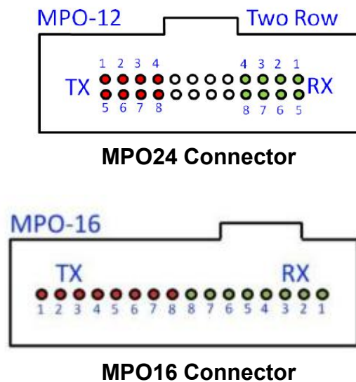
Figure 4. MPO24 and MPO16 Optical Receptacle and Channel Orientation
