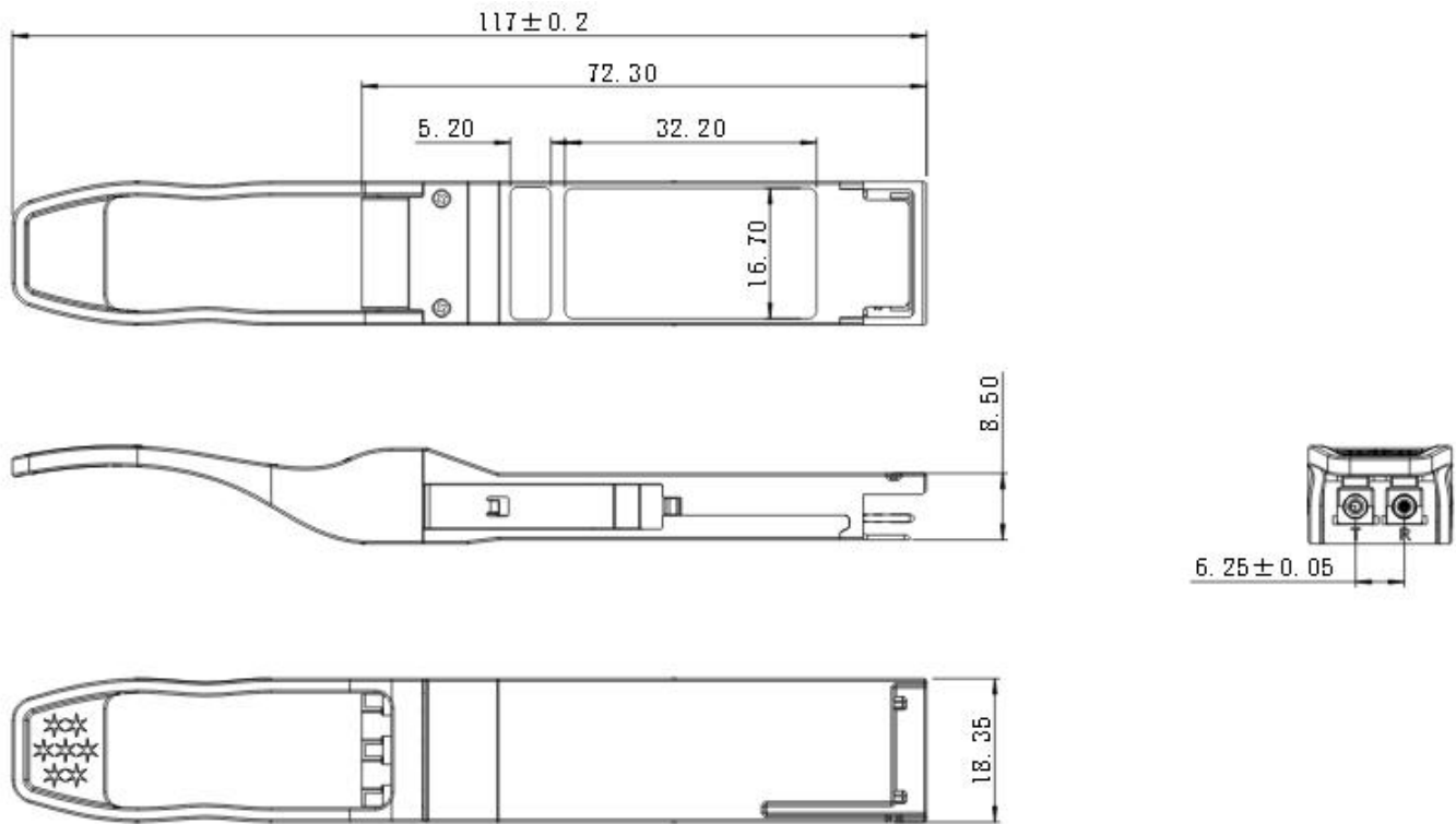
Figure 8. Mechanical Specifications
