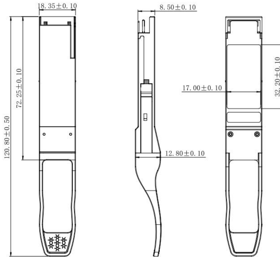
Figure6. Mechanical Specifications
