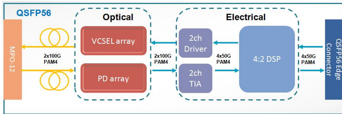
Figure1. Module Block Diagram
