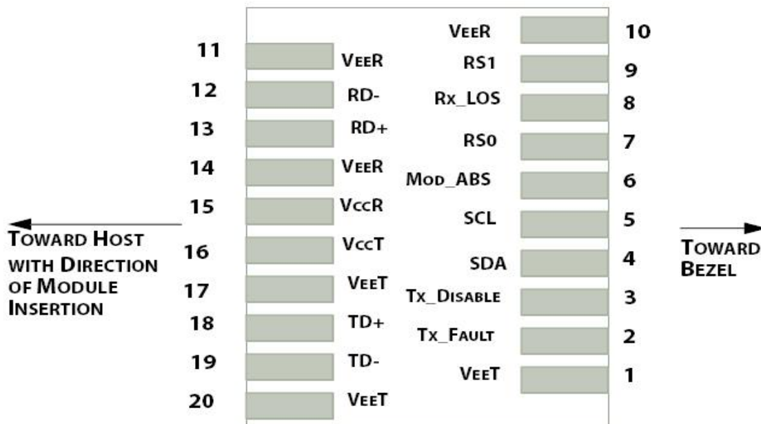
Figure2.Electrical Pin-out Details
