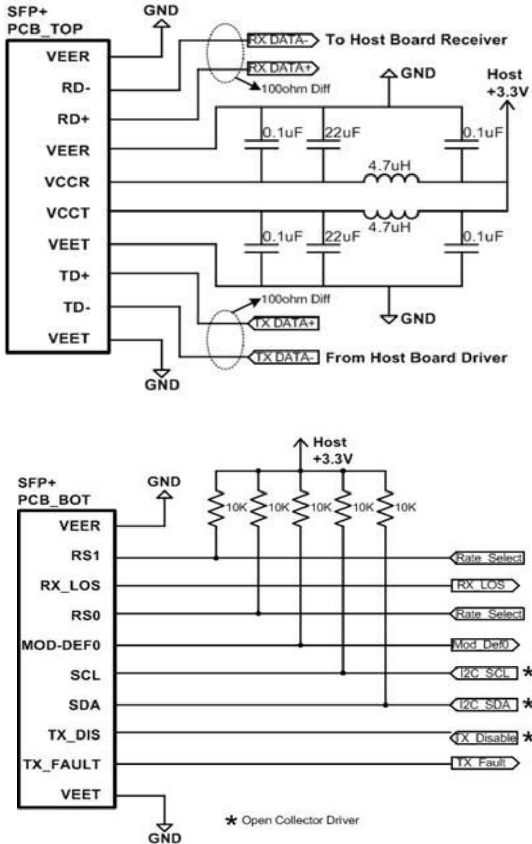
Figure3. Recommended Interface Circuit
