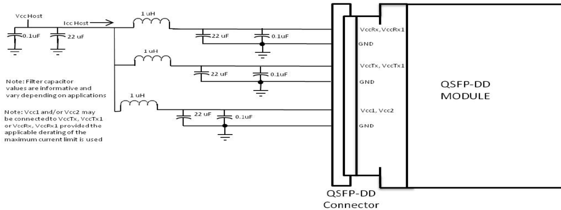
Figure4. Host Board Power Supply Filtering
