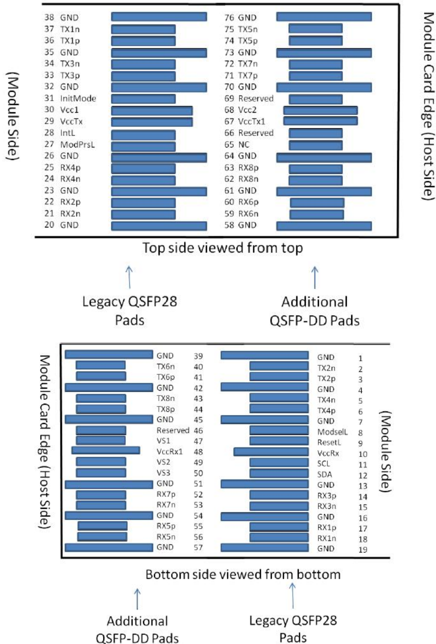
Figure3. Electrical Pin-out Details
