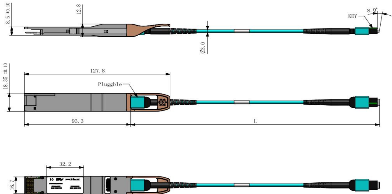
Figure7. Mechanical Specifications
