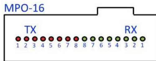
Figure 5. Optical Receptacle and Channel Orientation
