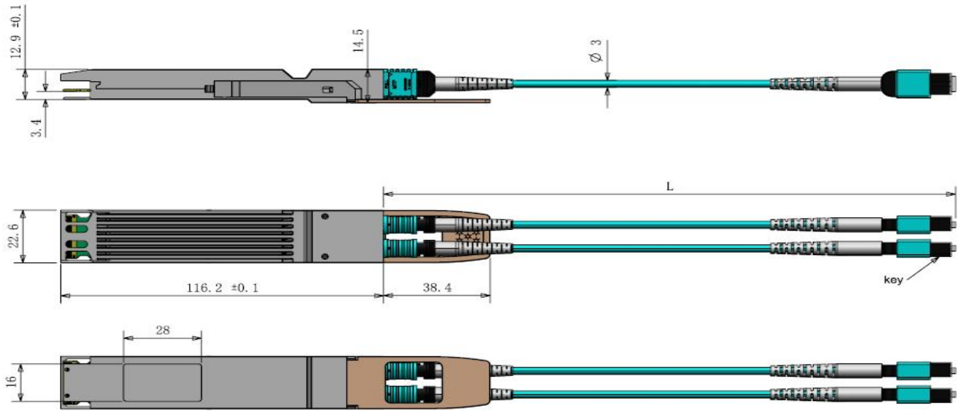
Figure7. Mechanical Specifications
