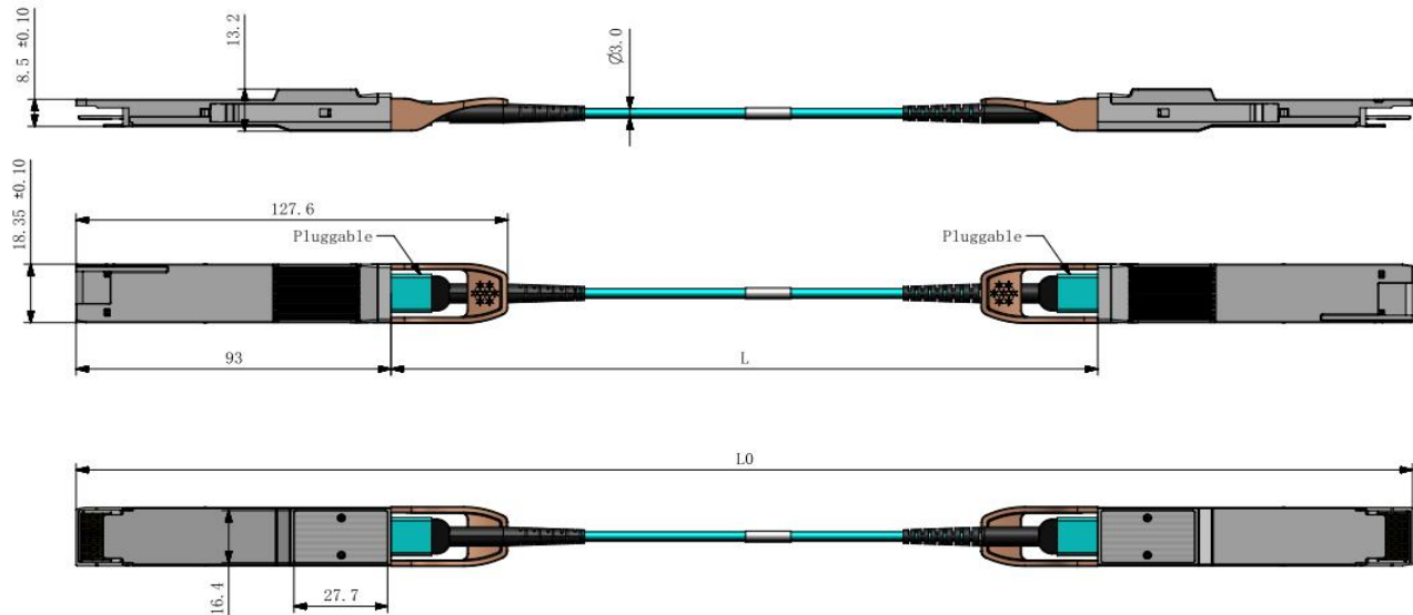
Figure7. Mechanical Specifications
