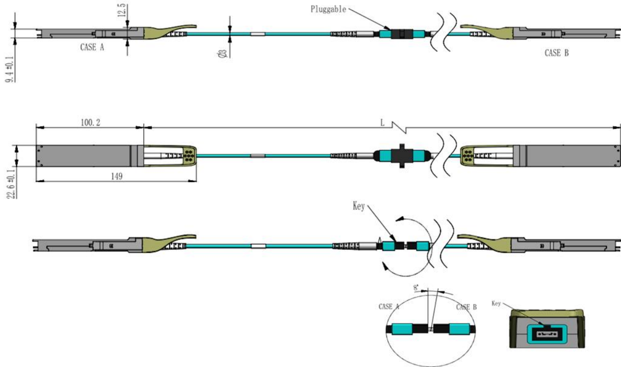
Figure 7. Mechanical Specifications
