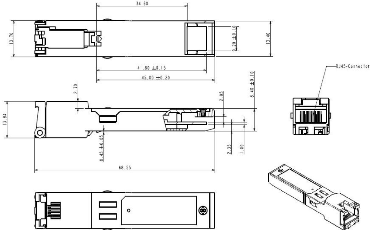
Figure 2. GE-FB-PxRT mechanical dimensions
