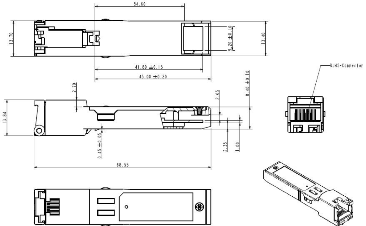
Figure 2. GE-FB-PxRC mechanical dimensions
