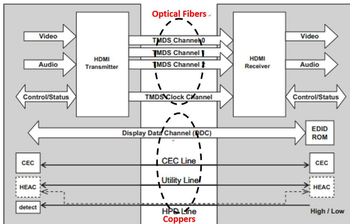
Figure 1. HDMI 2.0 AOC Block Diagram
