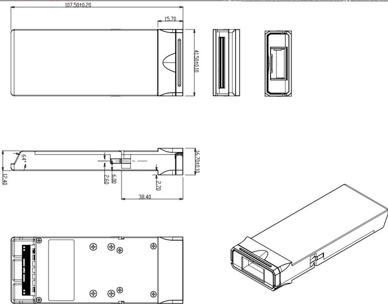
Figure4.Mechanical Specifications
