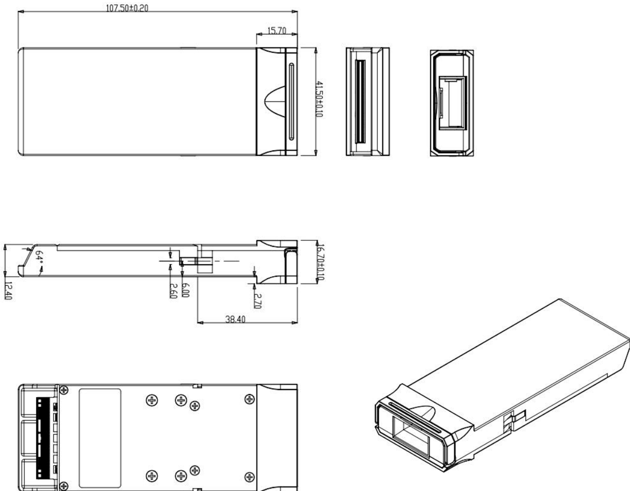
Figure4.Mechanical Specifications
