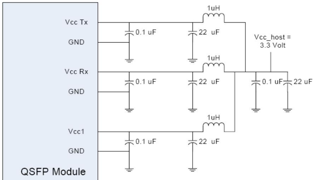
Figure 3. Host Board Power Supply Filtering
