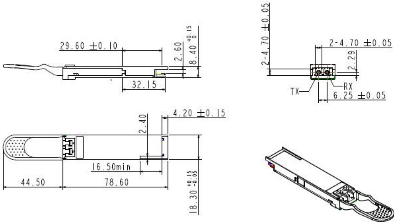
Figure 8. Mechanical Specifications
