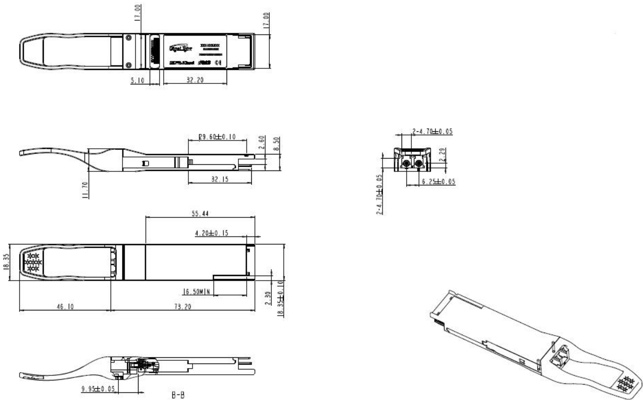
Figure 9. Mechanical Specifications
