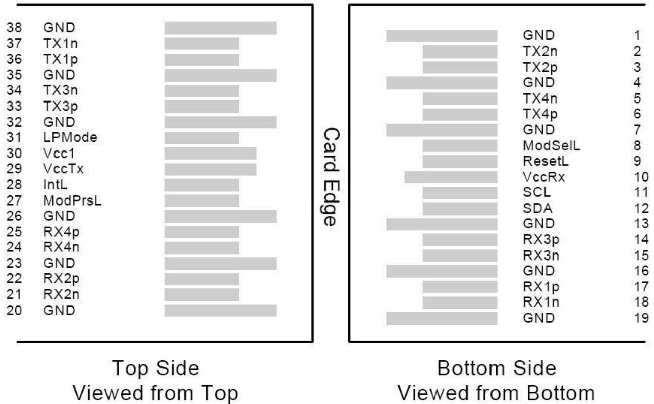
Figure 3. Electrical Pin-out Details
