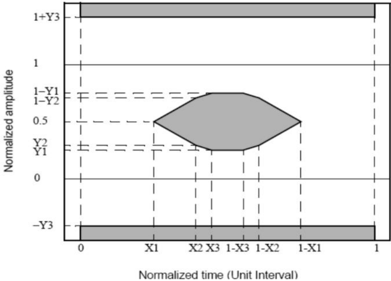
Figure 2. Eye Mask
