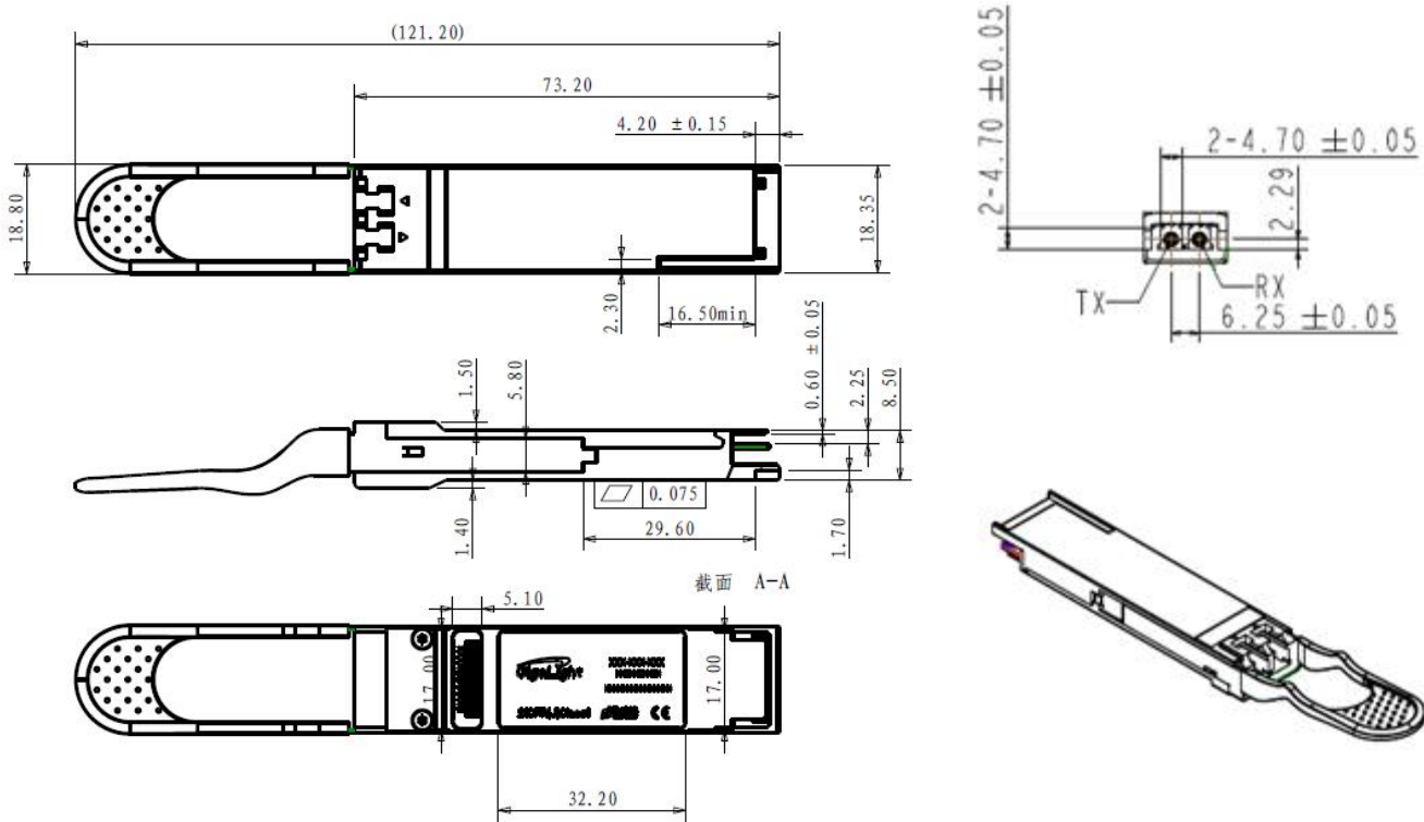
Figure10. Mechanical Specifications
