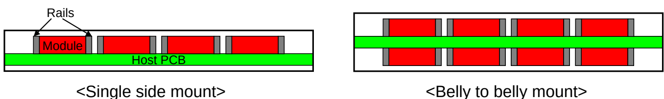
Figure 8-1: Mounting of CFP MSA module
