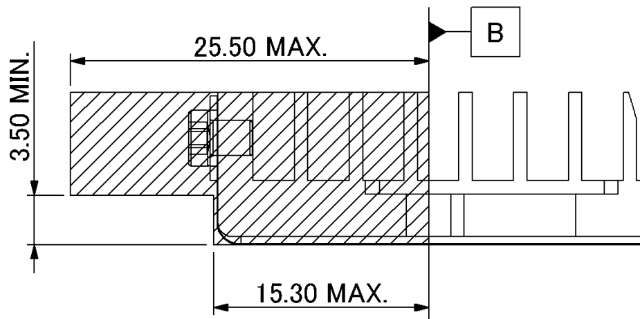
Figure 5-12: Riding Heat Sink Detail A
