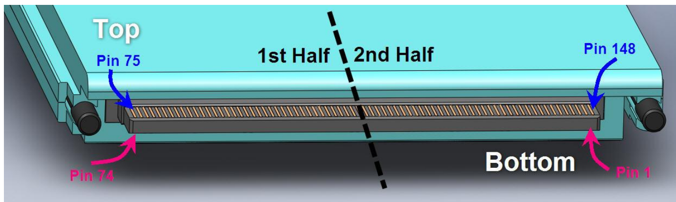
Figure 5-18: CFP Pin Map Orientation
