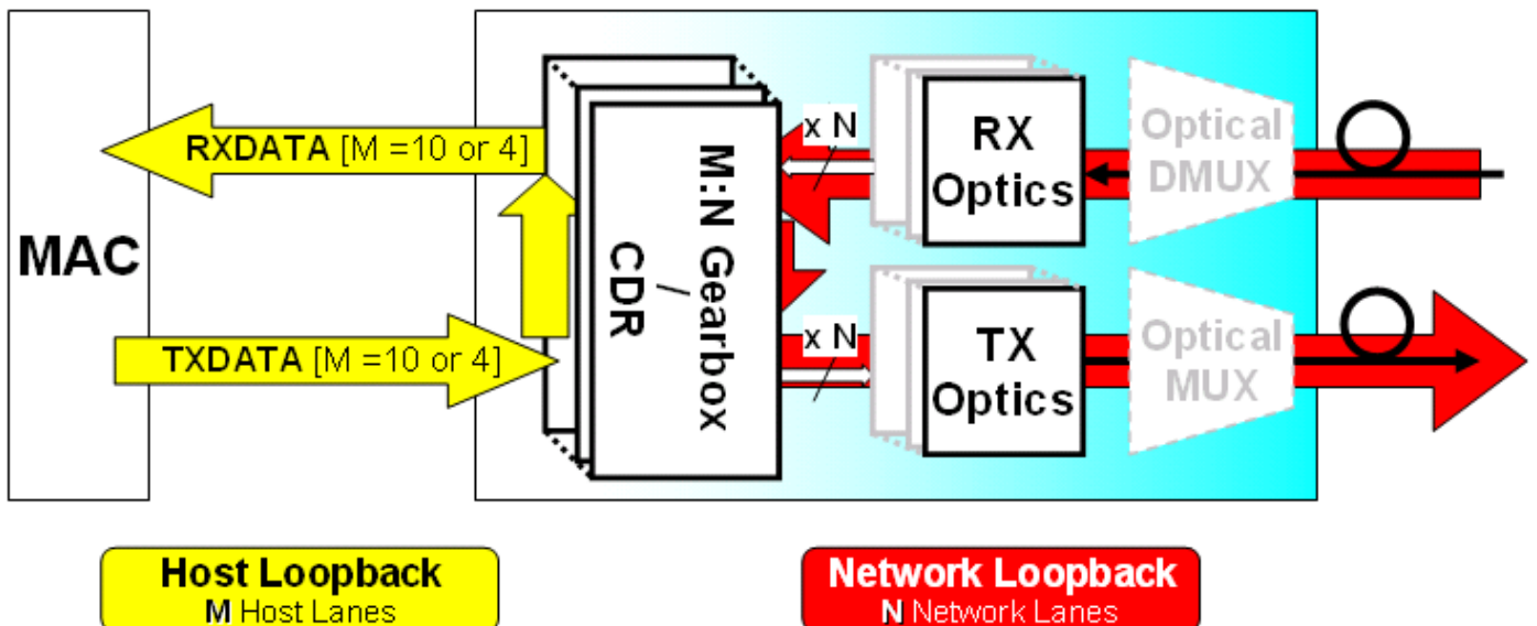
Figure 4-2: Optional Loopback Orientation
