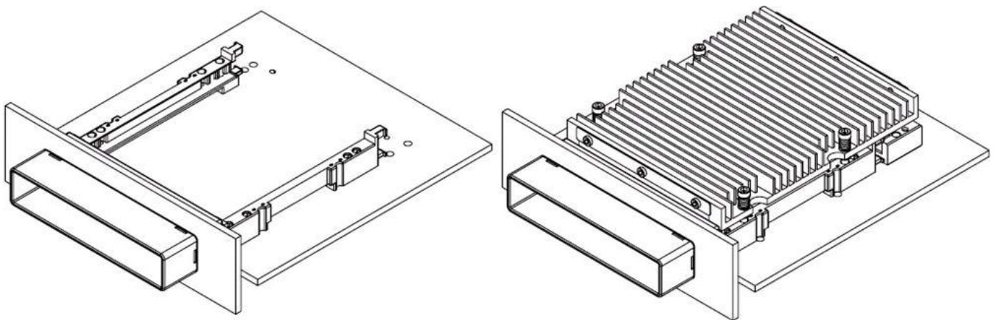
Figure 5-10: Riding Heat Sink Overview
