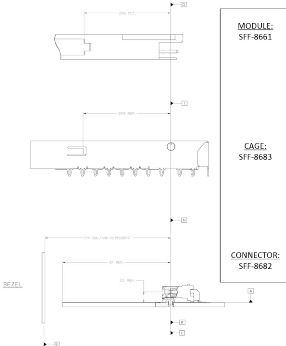
FIGURE 4-1 DATUM DEFINITIONS
